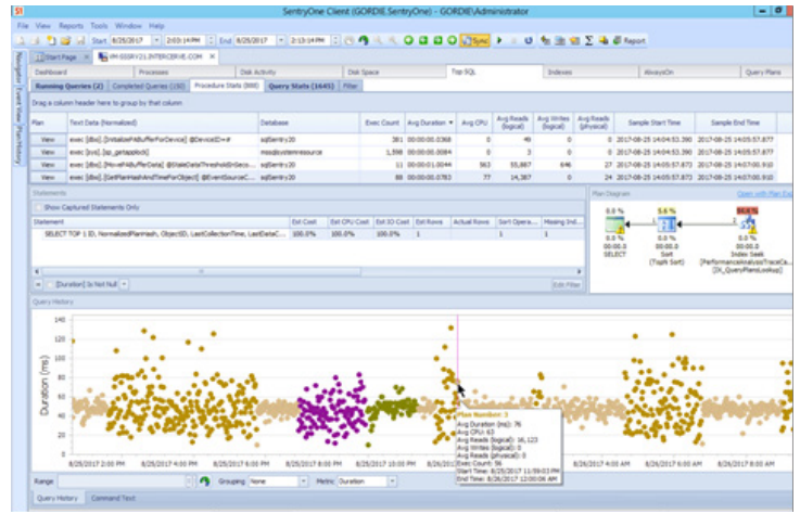
Figure 3 – The SQLSentry TopSQL feature provides instant visibility into which queries, and plans are consuming the most I/O, which simplifies and speeds the performance troubleshooting process.
